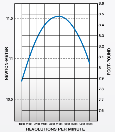
Net Torque
