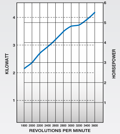
Net Power
